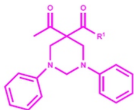
Hexahydropyrimidines
