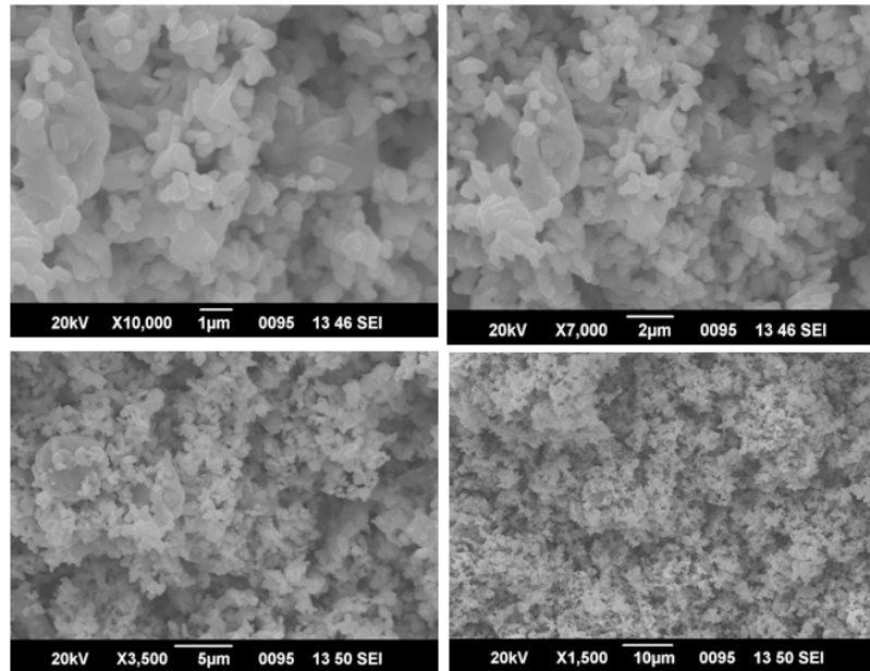
Fig.2. SEM images of sample \text{Sr}_{0.8}\text{Ba}_{0.2}\text{Fe}_{11.7}\text{La}_{0.2}\text{O}_{19}
