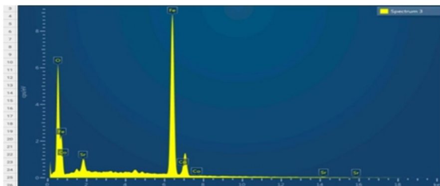
Fig Agraph of EDAX composition of \text{Sr}_{0.8}\text{Ba}_{0.2}\text{Fe}_{11.8}\text{Al}_{0.2}\text{O}_{19}
