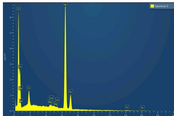
Fig.3. A graph of EDAX composition of \text{Sr}_{0.8}\text{Ba}_{0.2}\text{Fe}_{11.7}\text{La}_{0.2}\text{O}_{19}
