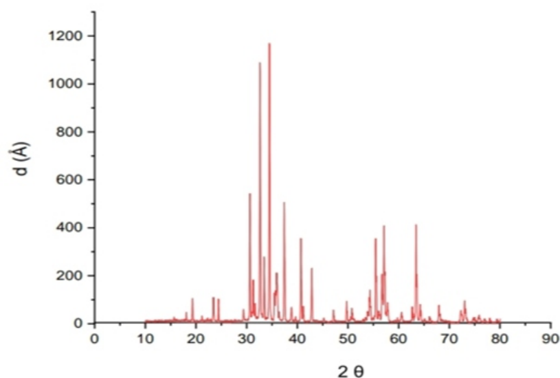
Fig.1. XRD graph of sample \text{Sr}_{0.8}\text{Ba}_{0.2}\text{Fe}_{11.7}\text{La}_{0.2}\text{O}_{19}
