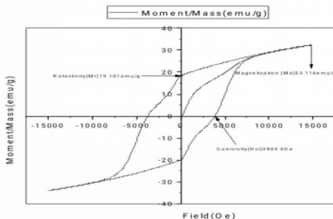
Fig Agraph of VSM OF \text{Sr}_{0.8}\text{Ba}_{0.2}\text{Fe}_{11.8}\text{Al}_{0.2}\text{O}_{19}
